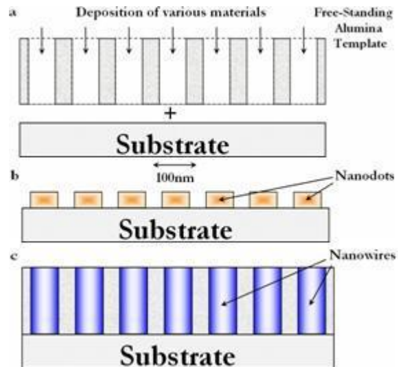
Figure 7 - Application of nanoporous alumina template in nanodot and nanowire synthesis.
