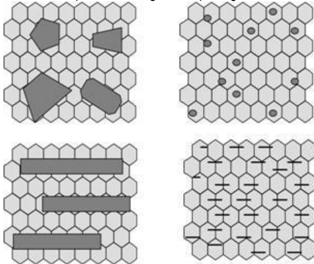
Figure 4 - Examples of nano-composite electrodeposits.
