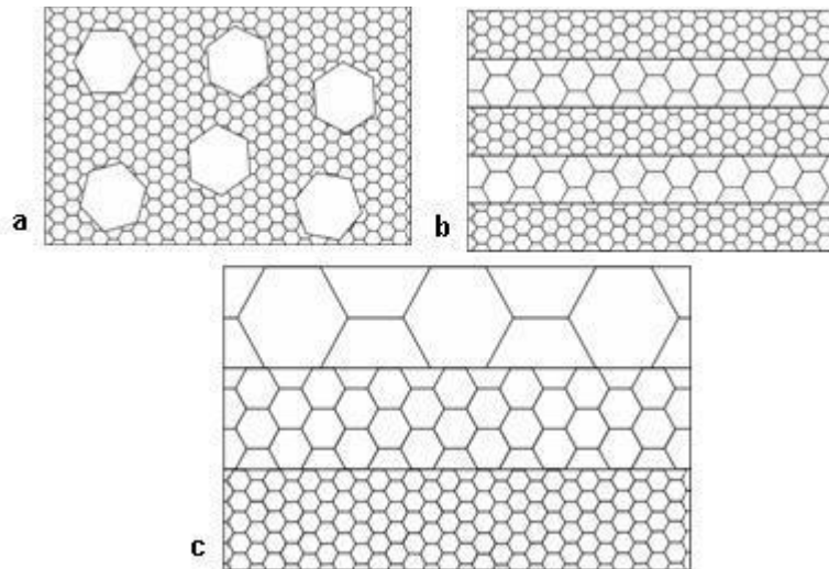
Figure 3 - Schematic diagrams showing various types of structurally graded nanomaterials: a) bimodal grain size distribution, b) alternate layers with different grain sizes and c) grain size gradient structure.
