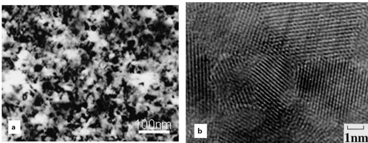
Figure 2 - Bright field (a) and high resolution (b) electron micrographs of nanocrystalline Ni with equiaxed grain shape and narrow grain size distribution.
